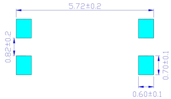
Recommended PCB solder PAD
